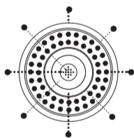
Submarine cable
